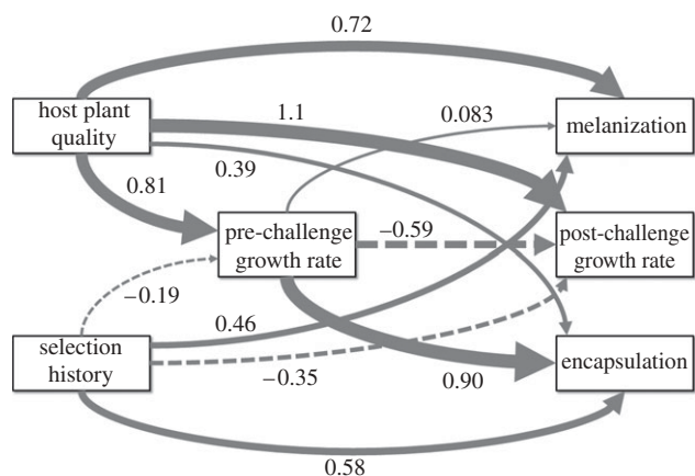
Figure 1. Structural equation model (path diagram) for the direct effects of host plant quality and selection history on melanization, encapsulation and post-challenge growth rates, and their indirect effects mediated through pre-challenge growth rate. The levels of the dichotomous variables, host plant quality and selection history were assigned such that devil's claw = 0, tobacco = 1, domesticated laboratory population = 0 and wild field population = 1. The width of the path corresponds with the magnitude of the effect. Positive relationships are indicated by solid lines, and negative relationships by dashed lines. See table 1 for 95% CI of the path coefficient estimates.
